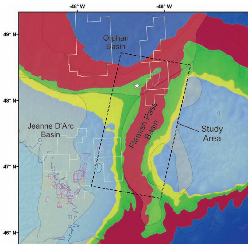
Figure 3: Dashed rectangle outlines the generalized location of the study area in Phase 1 of the NL Gas Hydrates Research Program. Outline of sedimentary basins shown by tan-colored lenses. Calculated stability zone thickness after (Majorowicz and Osadetz, 2003) and BSR observed by Mosher, 2011 (white star) are shown. See Figure 2 for location and legend.
