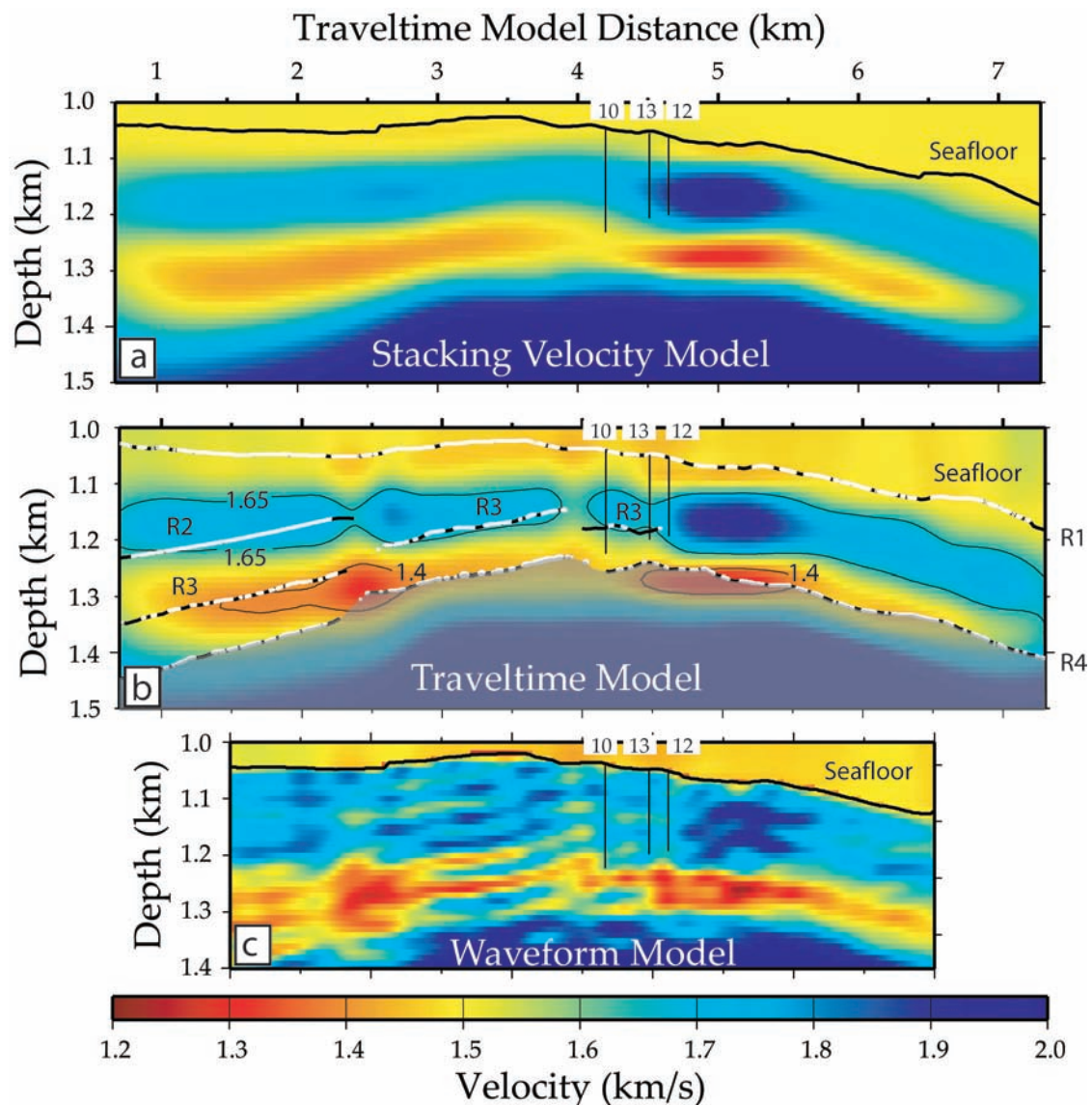
Figure 2: Velocity model evolution: a) Model from stacking velocity analysis, b) Model from a composite traveltime inversion – depth migration method (Jaiswal and Zelt, 2008), and c) Model from waveform inversion. The seafloor is labeled and the trajectory of Sites NGHP-01-10, 12, and 13 are overlain. Horizons R1 – R4 are used in modeling. Velocity greater than 1.65 km/s and less than 1.4 km/s respectively indicate hydrates and free gas.
