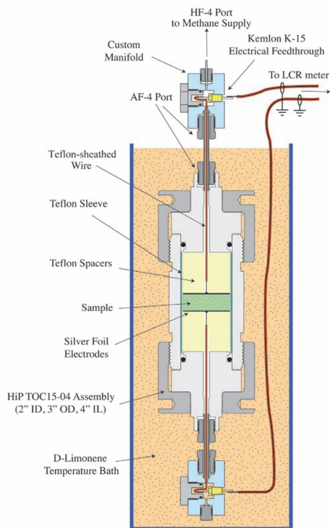
Figure 2: Pressure vessel used to synthesize \text{CH}_4 hydrate and measure conductivity.
